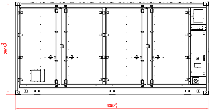
Right View
